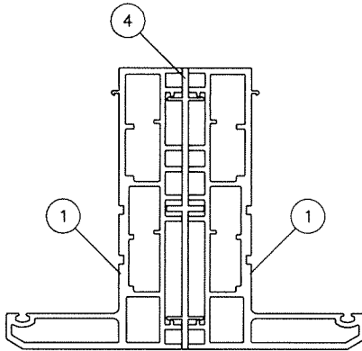
MULLION 'M'
